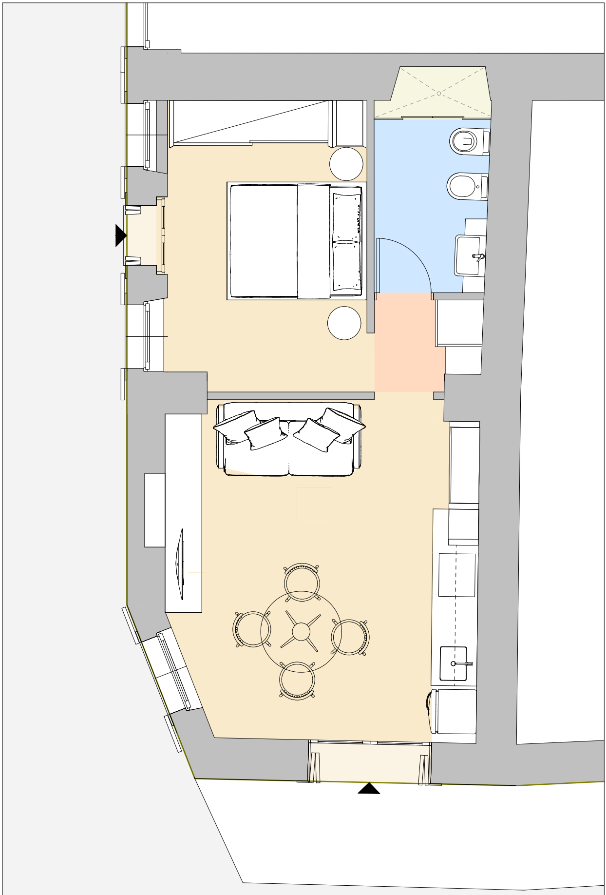
PIANO TERRA mq 47,96
